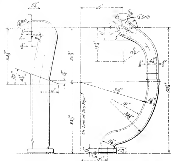
Fig. 2.—Method of Cutting and Welding Steam Pipes
